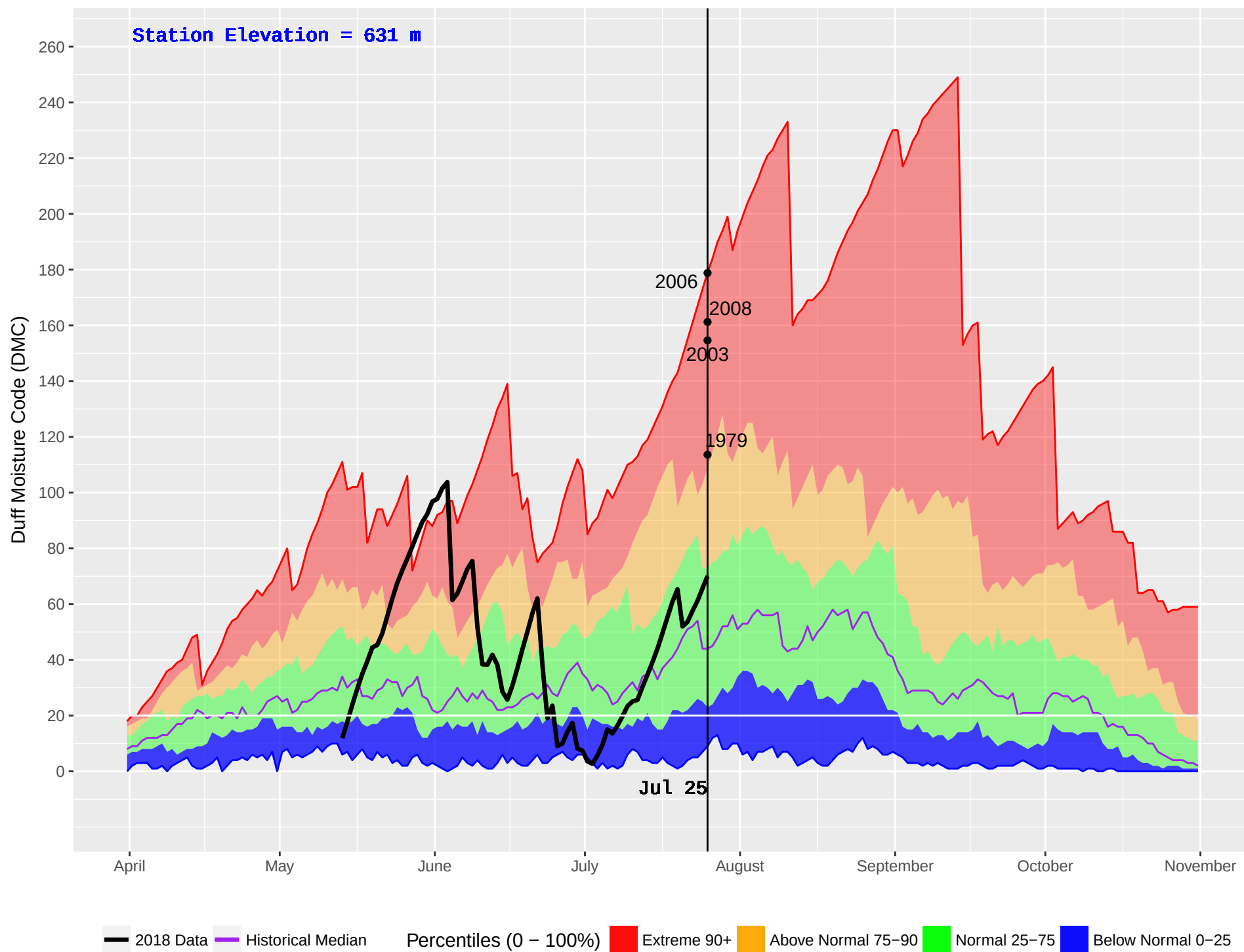
EAST BARRIERE (243) : Historical (1978–2016) and Current (2018) Noon Duff Moisture Code (DMC)
